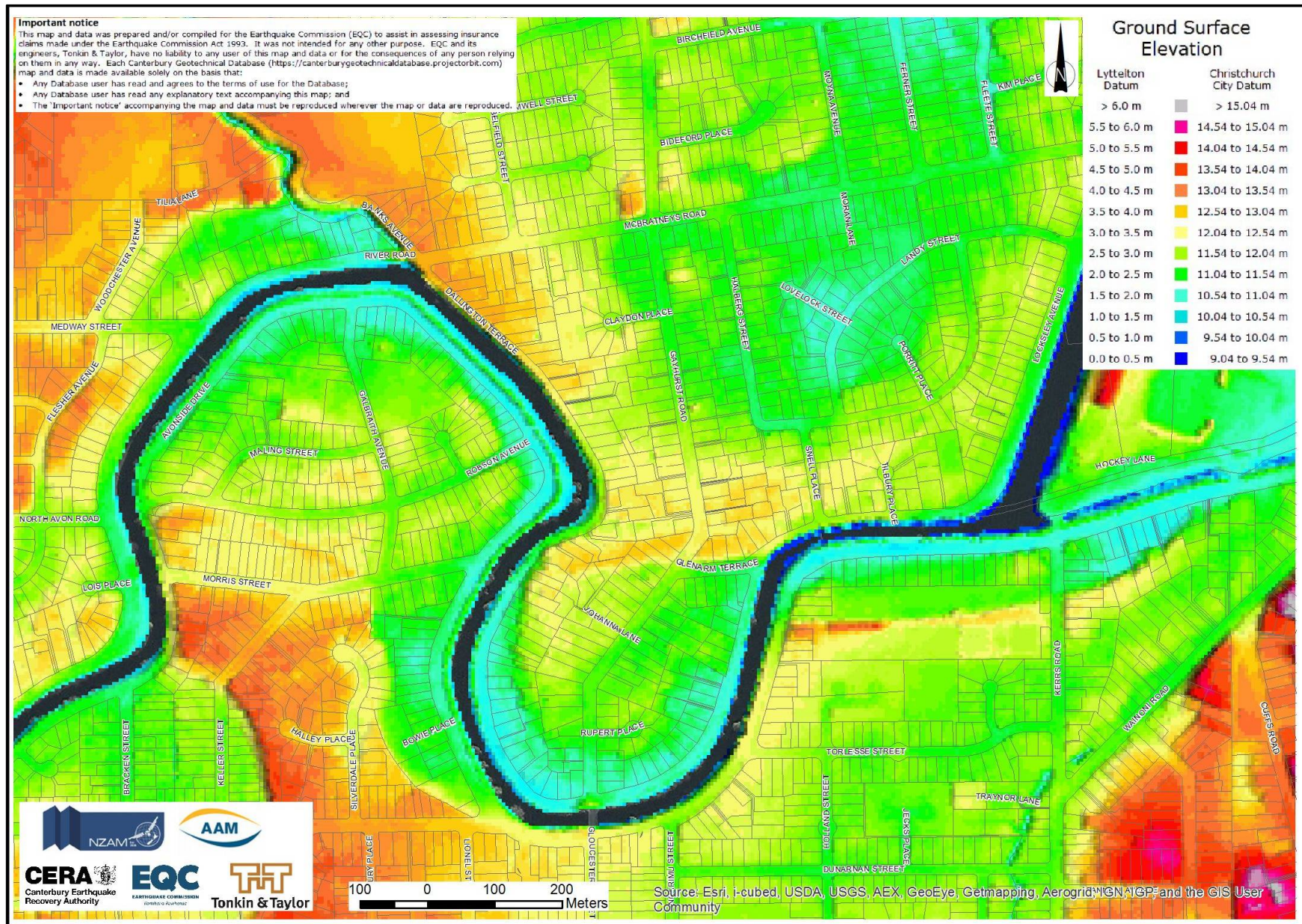
Figure 7 – Ground surface elevation from February 2012 survey
